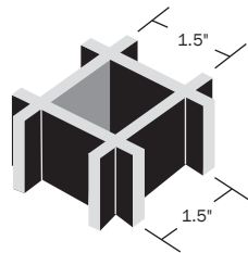
1" or 1½" thick, 1½" x 1½" Square Grid
