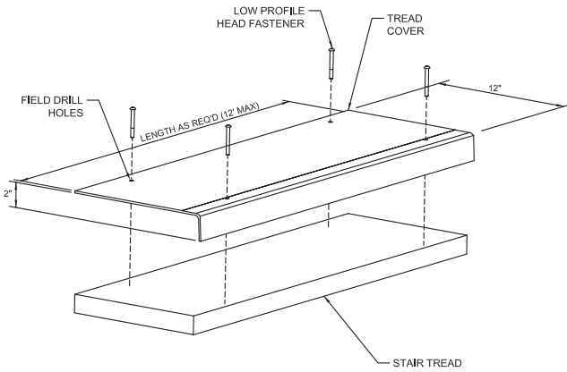
Cover Placement for Wood and Concrete Treads
