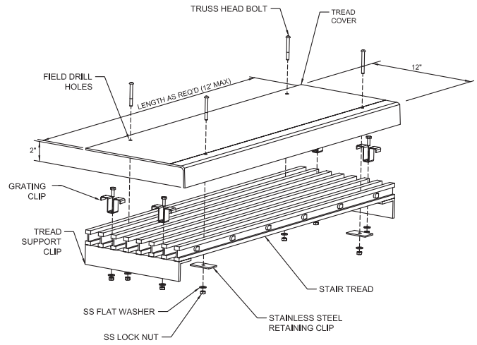
Cover Placement for Stair Tread Grating
